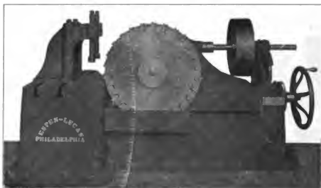
Fig. 4906. Cold Saw Cutting Off Machine, Fitted with Taylor-Newhold Cold Saw. Espin-Lucas Machine Works.
